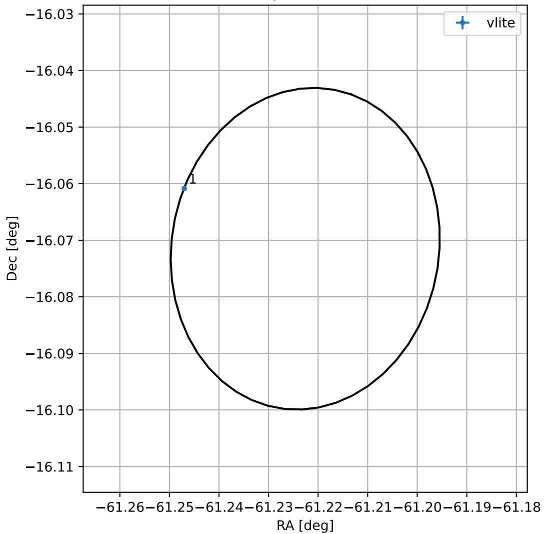
4FGL J1955.1-1604
