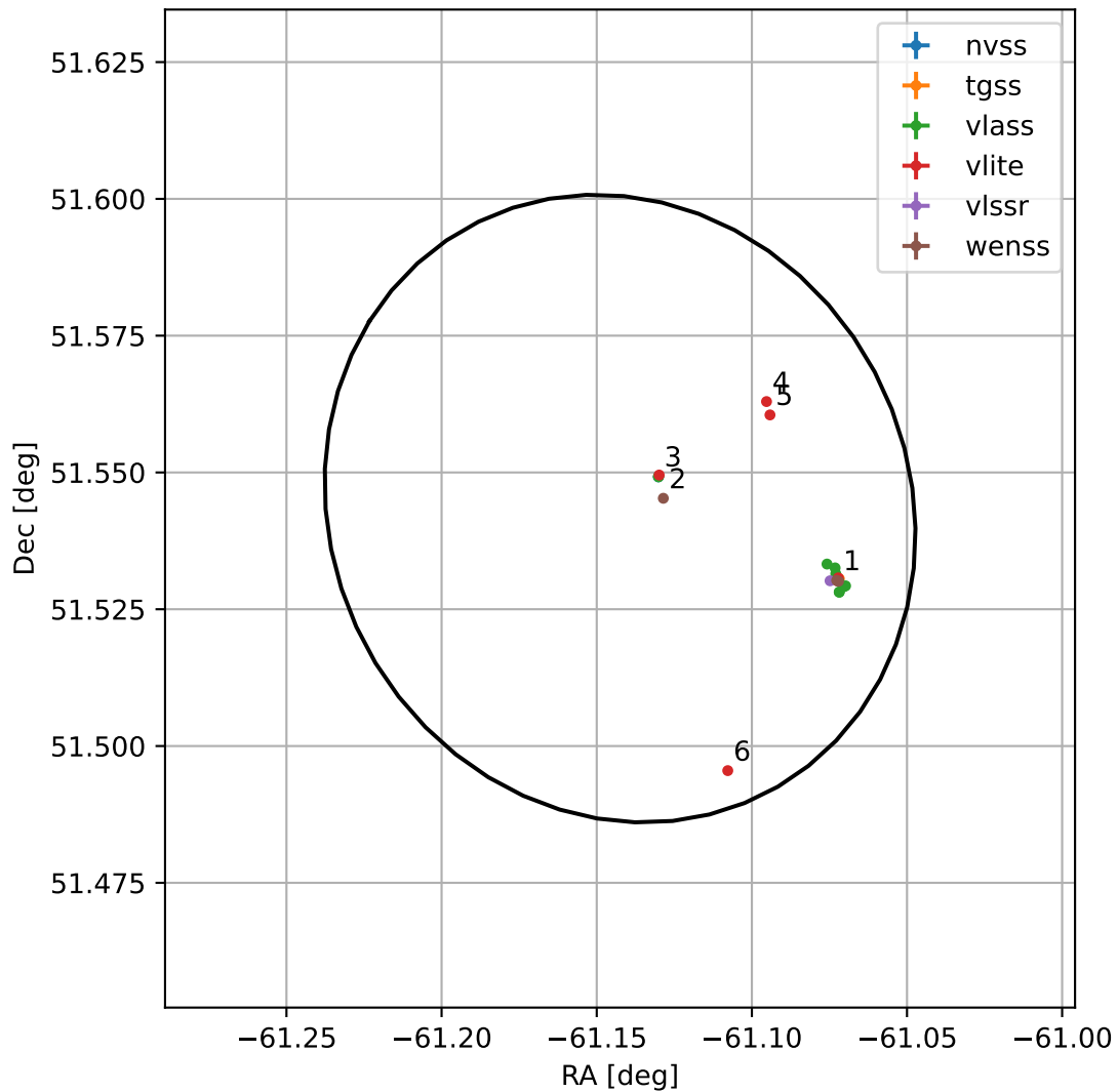
4FGL J1955.4+5132
