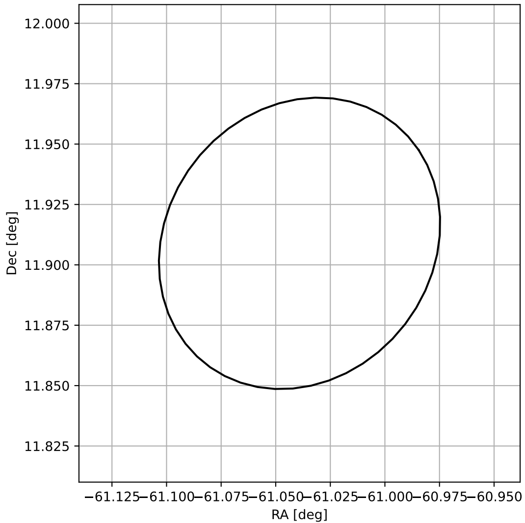
4FGL J1955.8+1154
