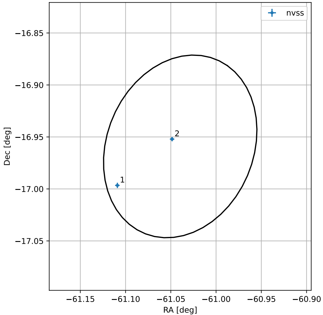
4FGL J1955.8-1657
