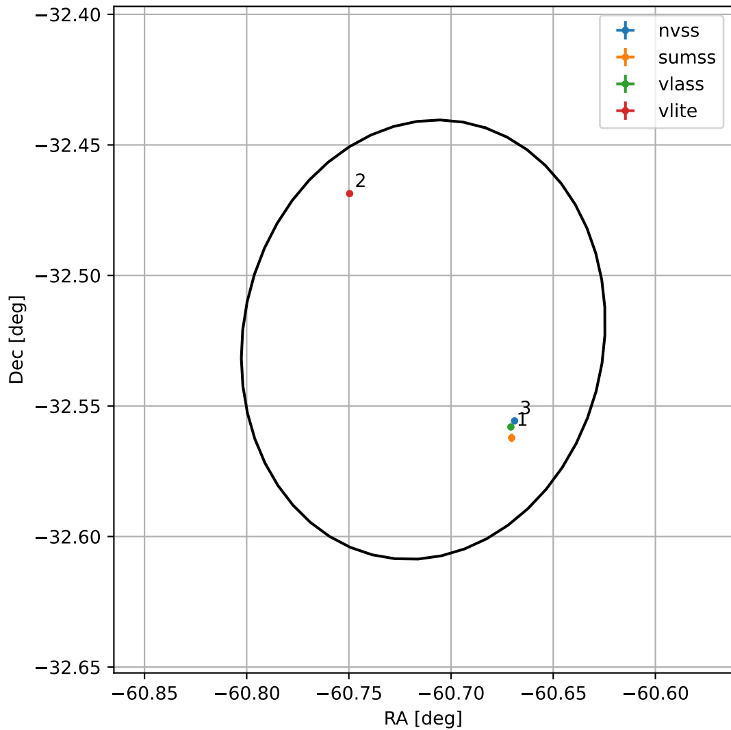
4FGL J1957.1-3231
