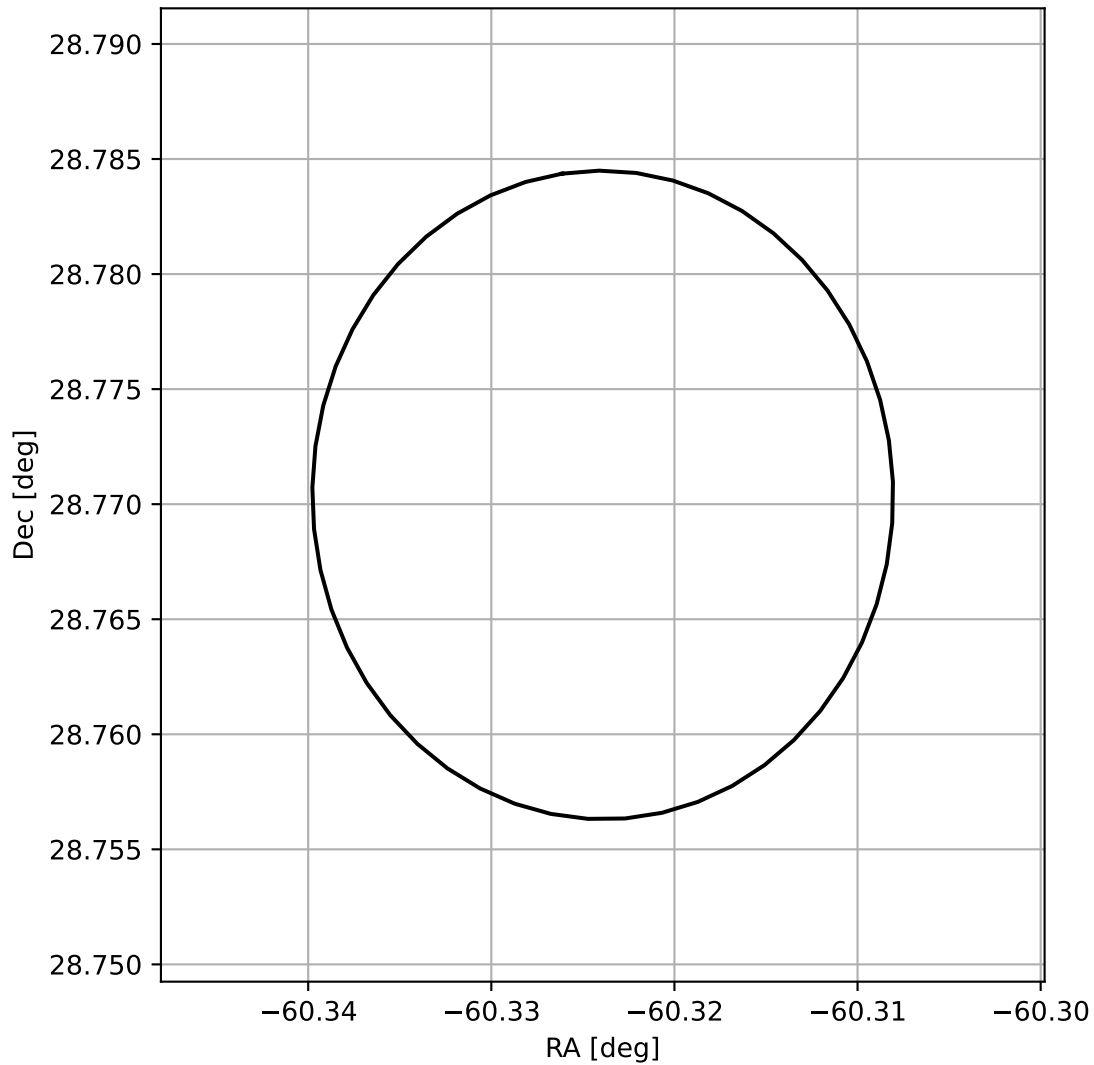
4FGL J1958.7+2846
