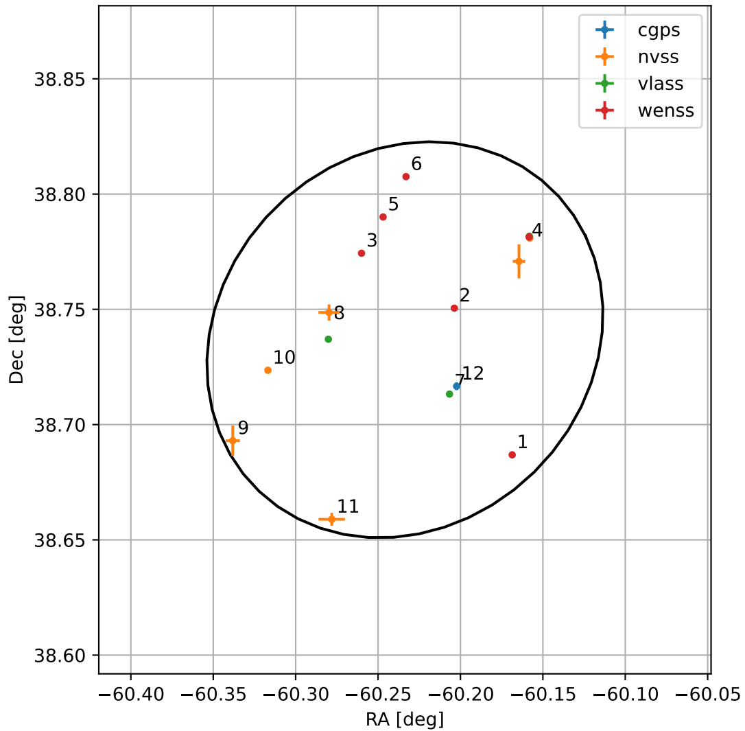
4FGL J1959.0+3844
