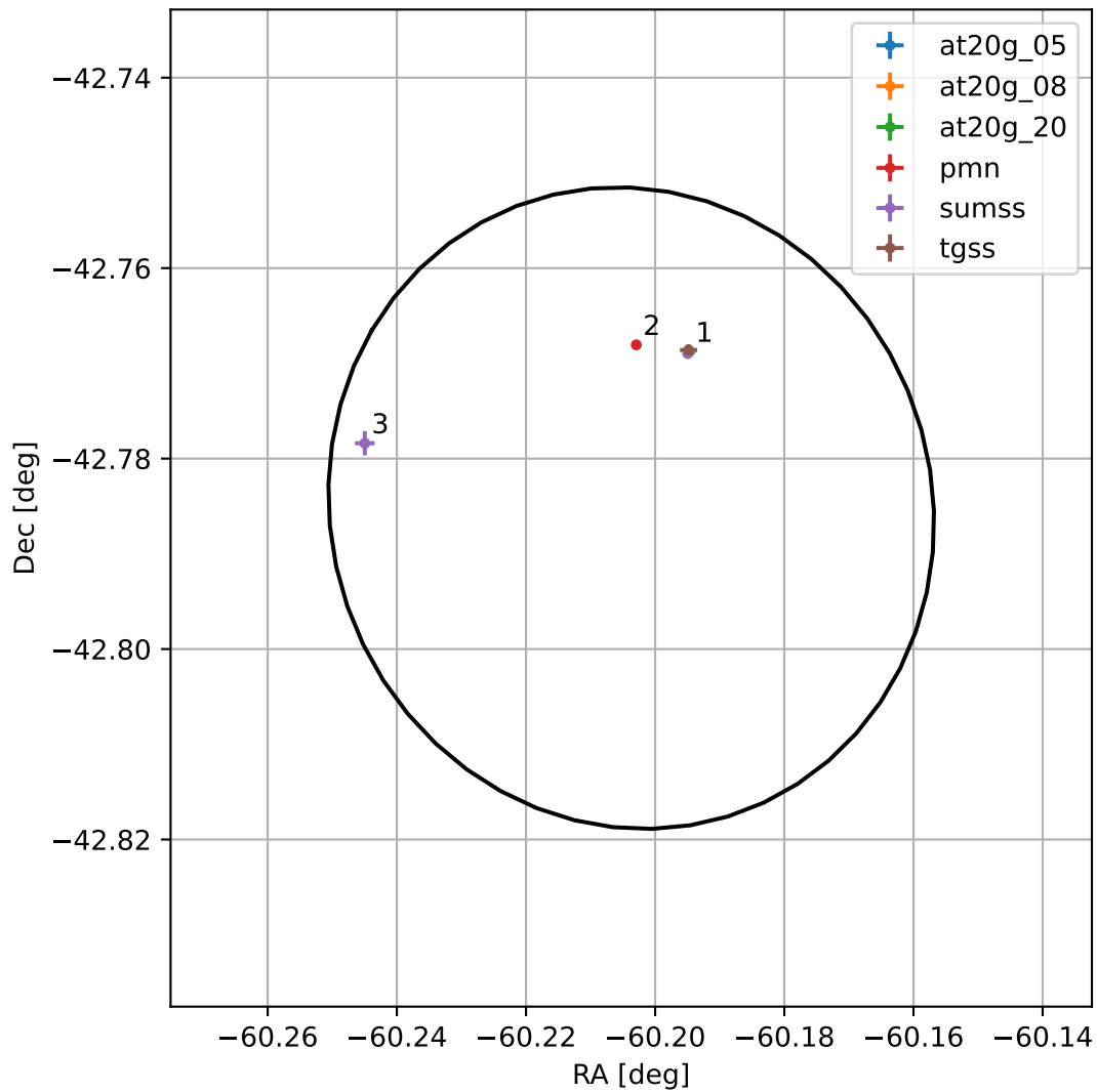
4FGL J1959.1-4247
