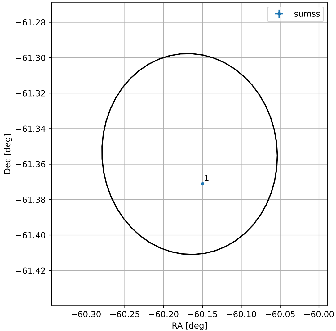
4FGL J1959.3-6121
