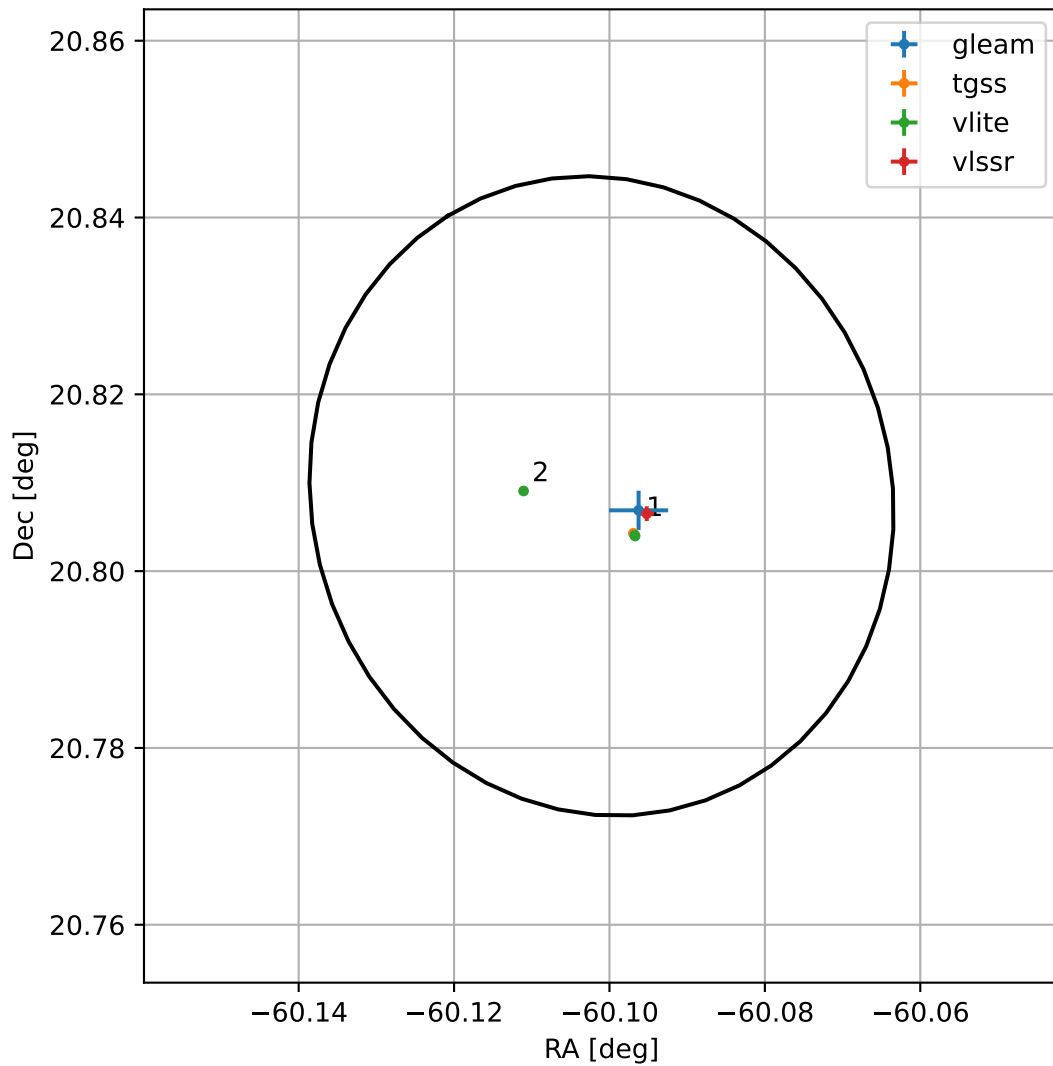
4FGL J1959.5+2048
