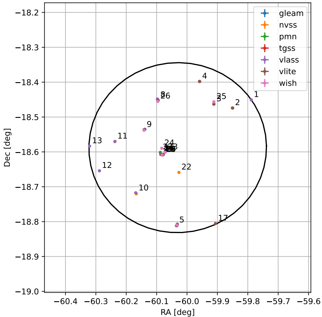
4FGL J1959.8-1835
