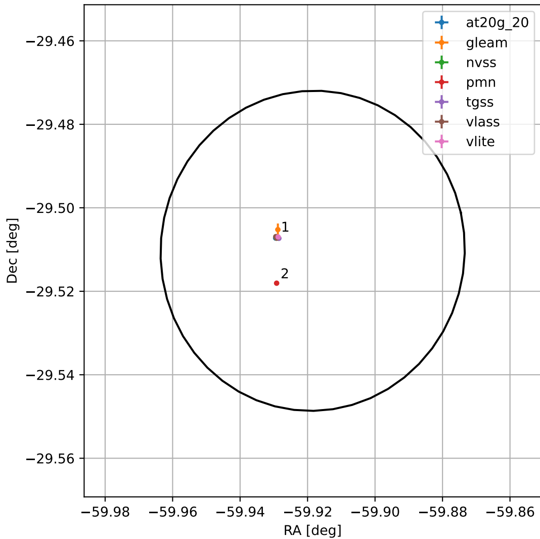
4FGL J2000.3-2930
