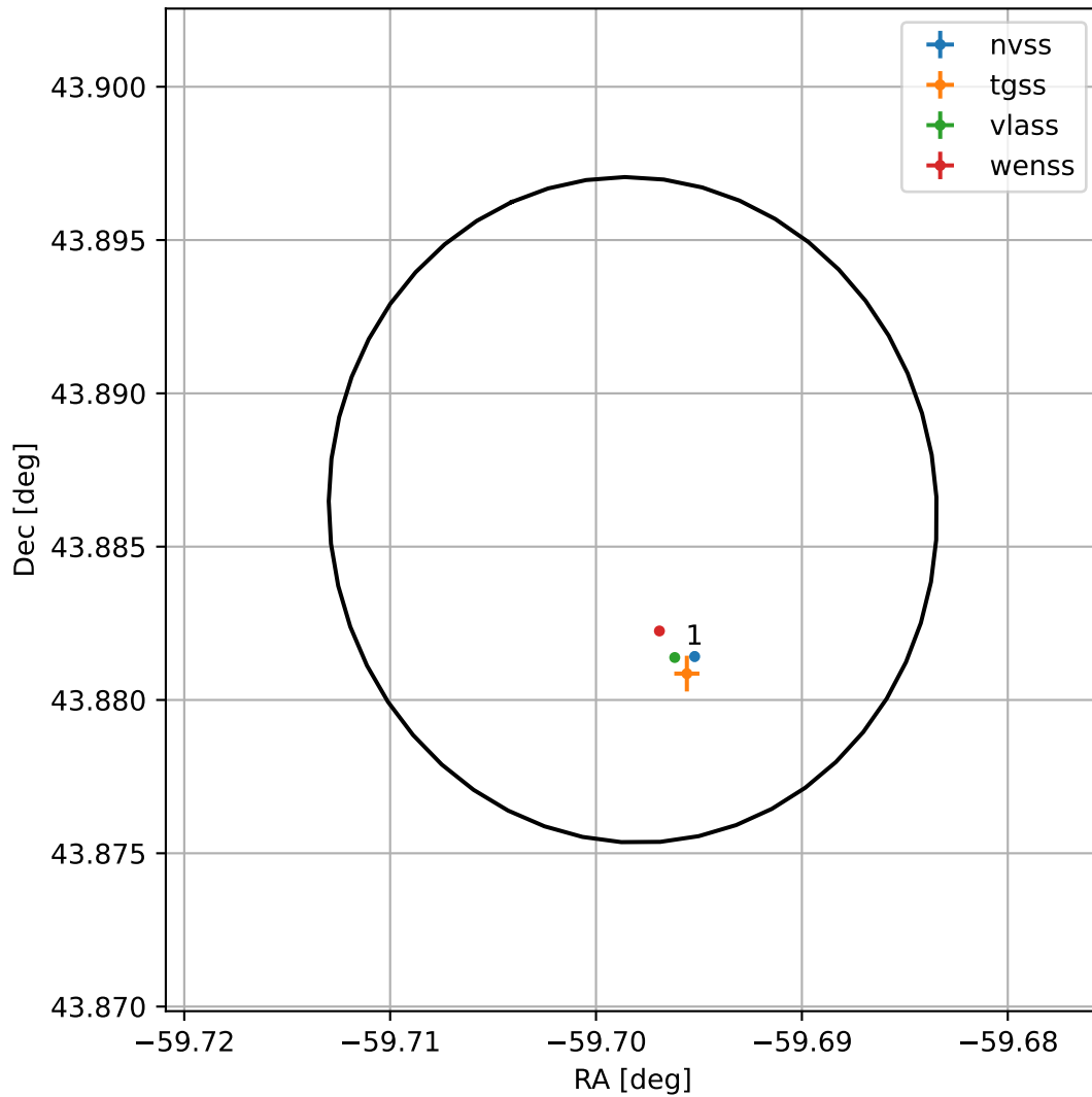
4FGL J2001.2+4353
