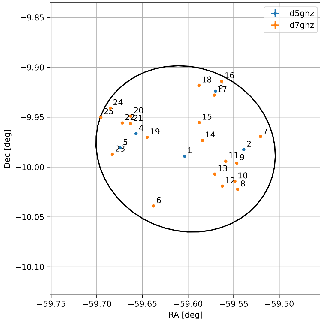
4FGL J2001.5-0958
