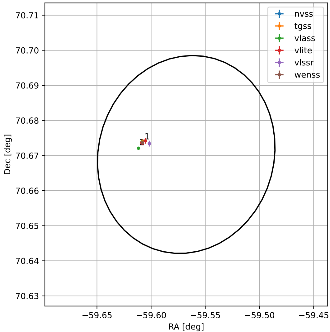
4FGL J2001.7+7040
