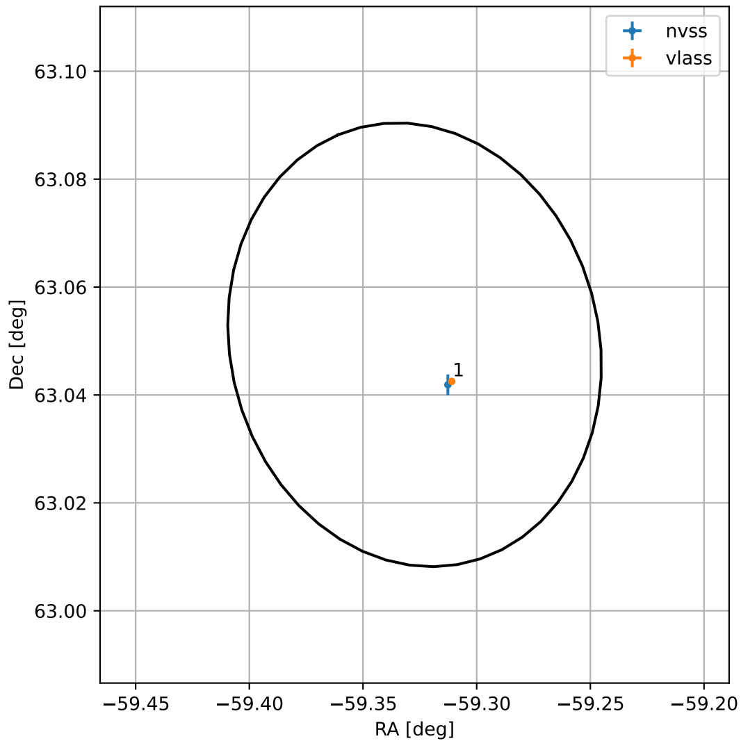
4FGL J2002.6+6302
