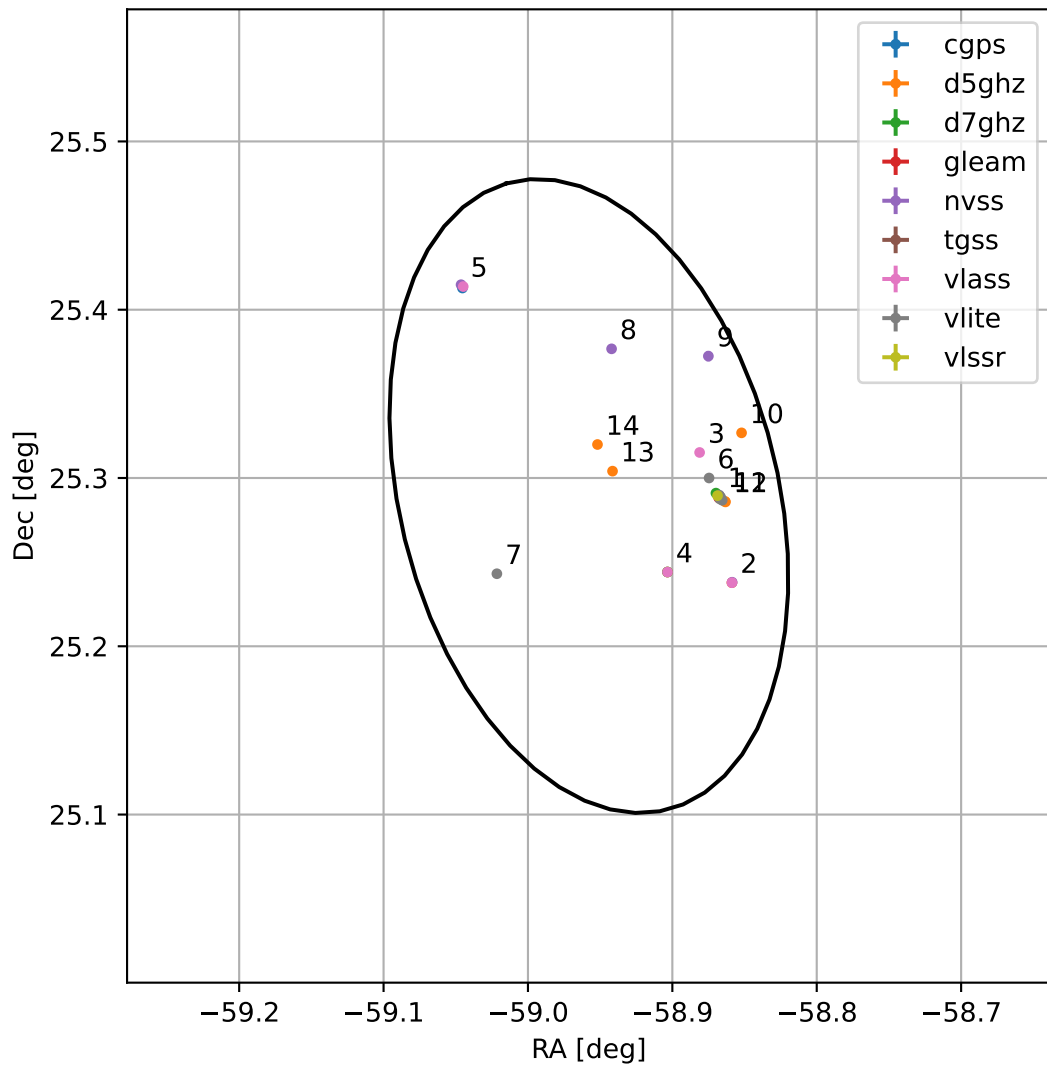
4FGL J2004.1+2517
