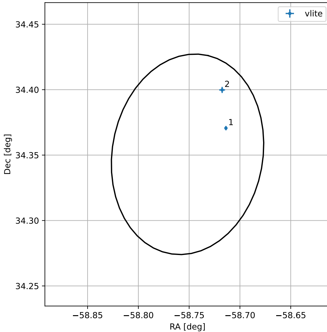
4FGL J2004.9+3421
