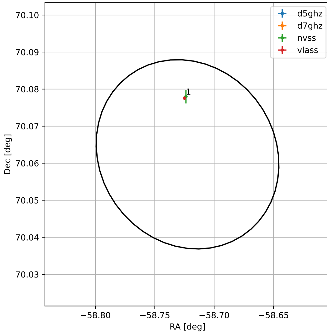
4FGL J2005.1+7003
