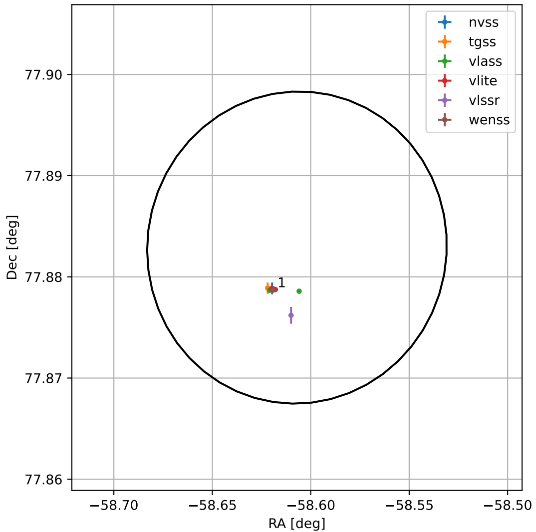
4FGL J2005.5+7752
