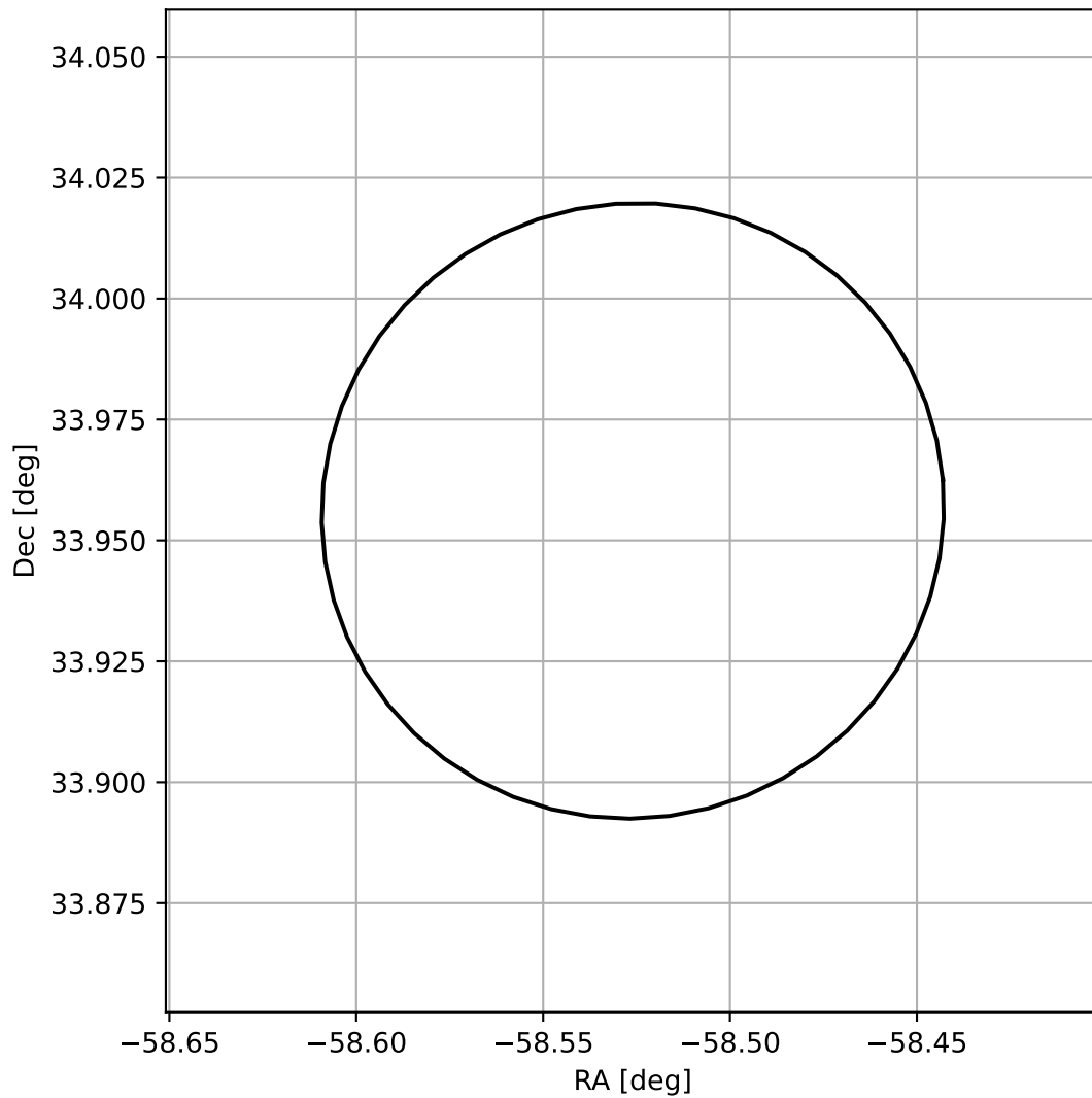
4FGL J2005.8+3357
