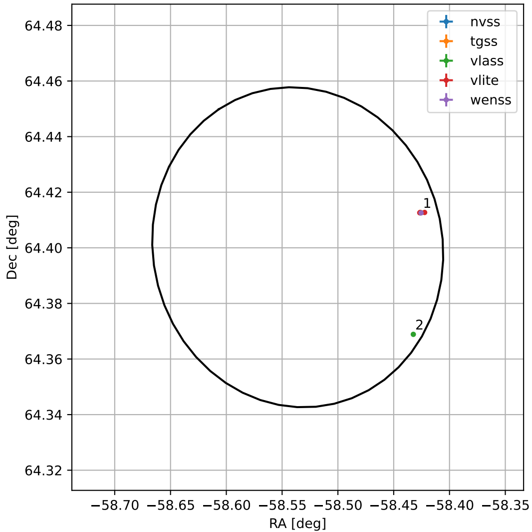
4FGL J2005.8+6424
