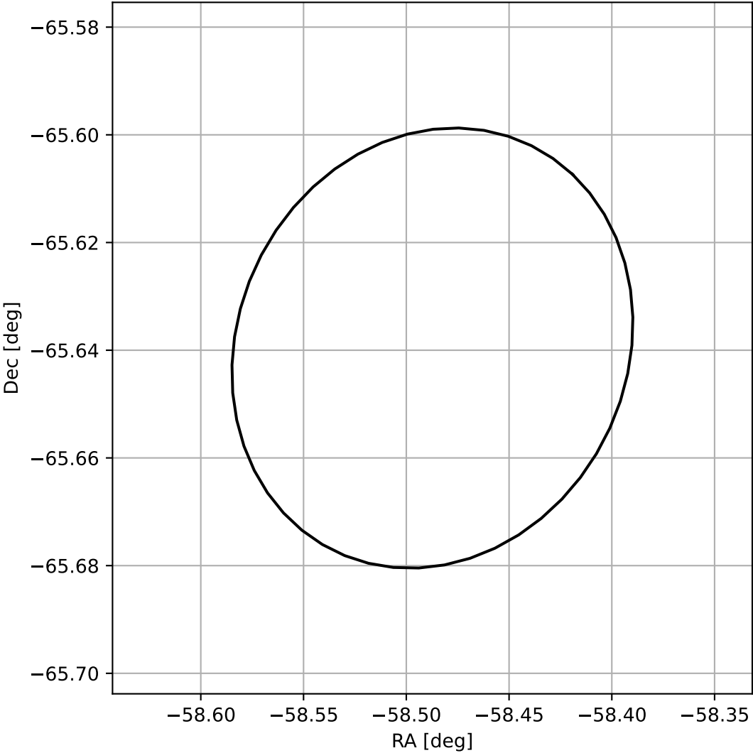
4FGL J2006.0-6538
