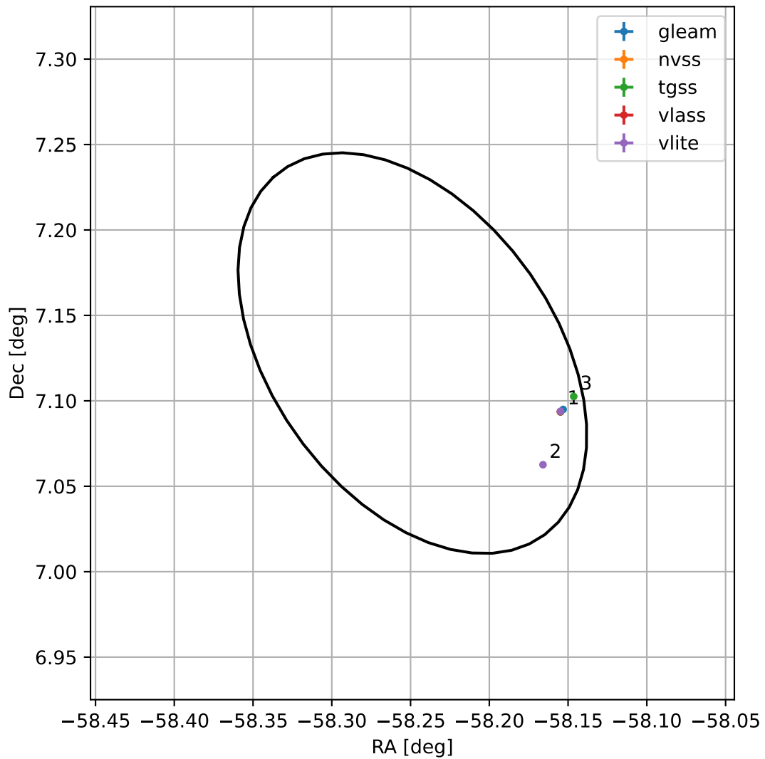
4FGL J2007.0+0707
