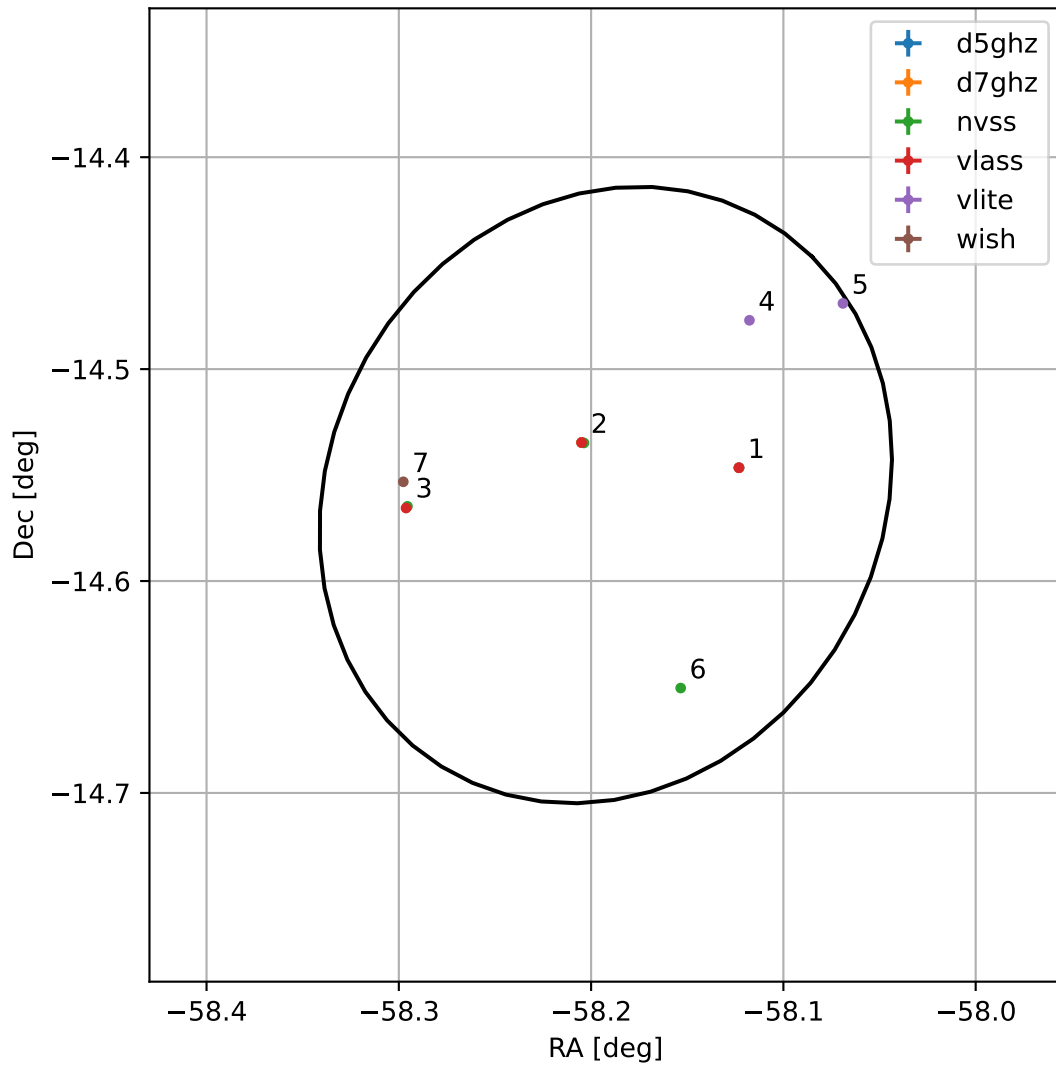
4FGL J2007.2-1433
