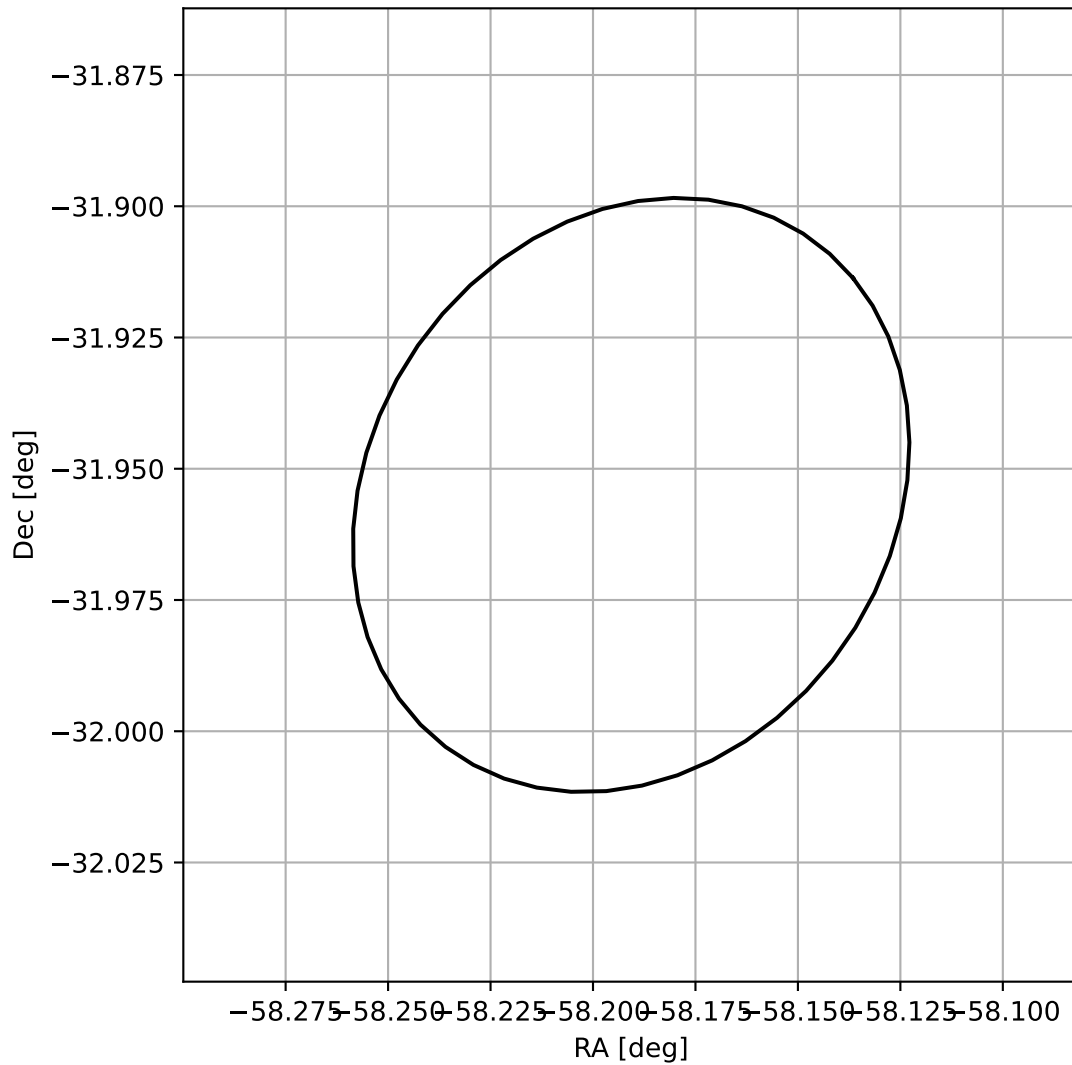
4FGL J2007.2-3157
