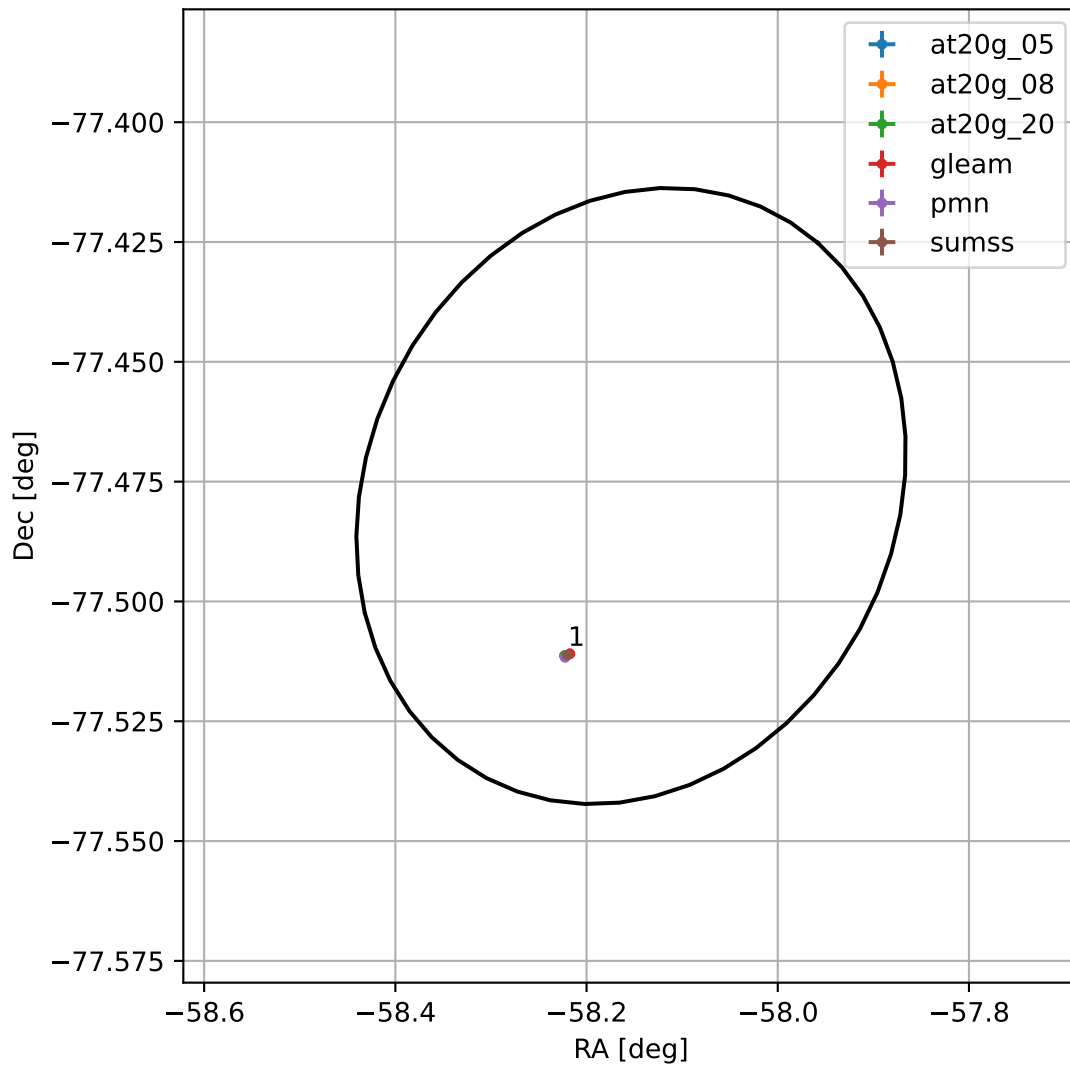
4FGL J2007.3-7728
