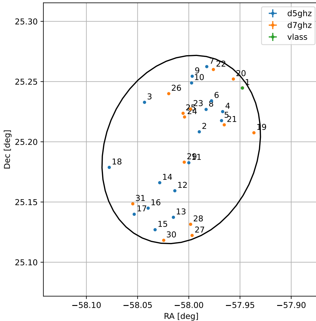
4FGL J2007.9+2511
