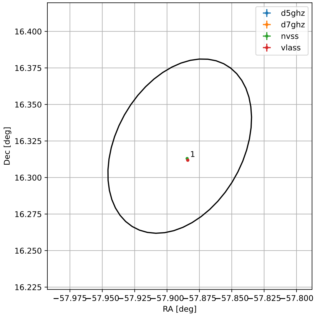
4FGL J2008.4+1619
