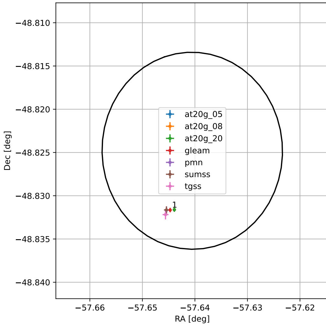
4FGL J2009.4-4849
