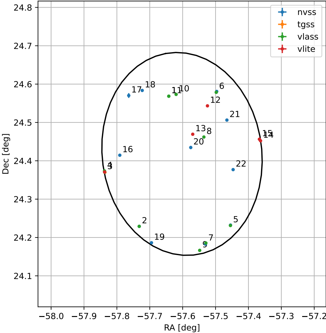
4FGL J2009.5+2425
