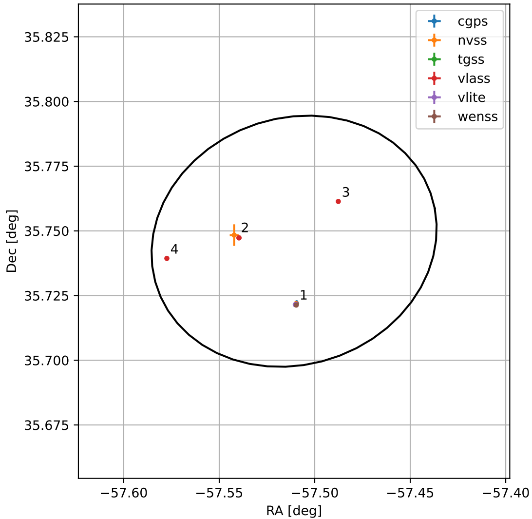
4FGL J2009.9+3544
