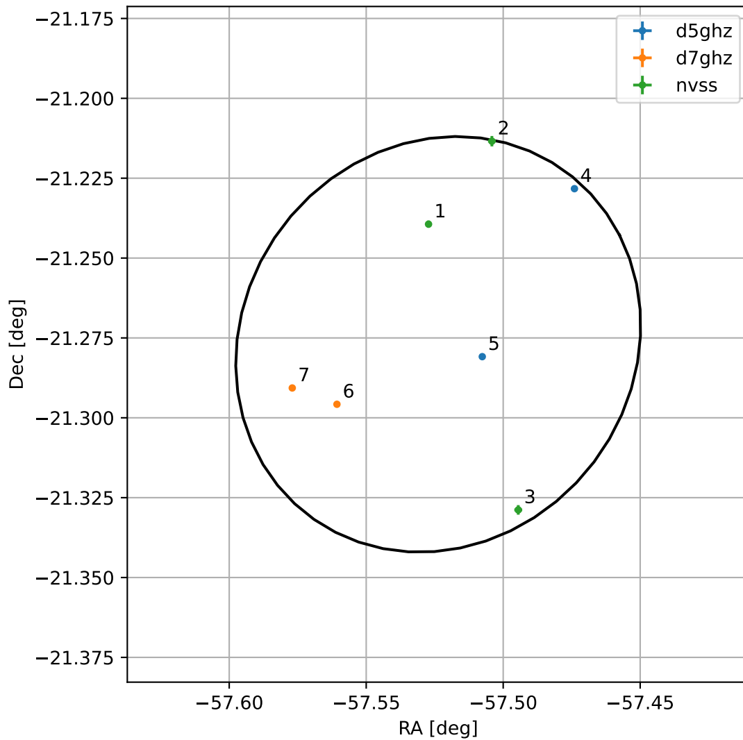
4FGL J2009.9-2116
