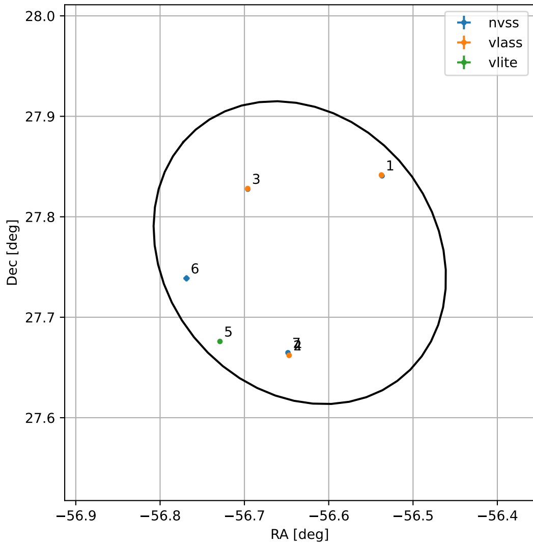
4FGL J2013.4+2745
