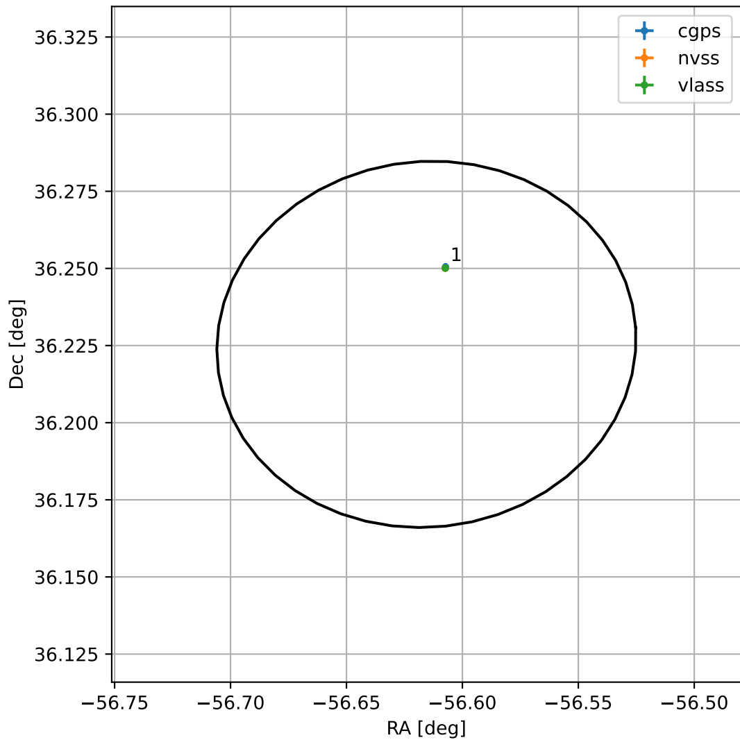
4FGL J2013.5+3613
