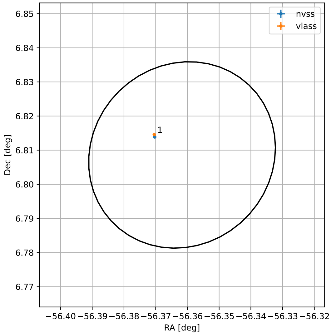
4FGL J2014.5+0648
