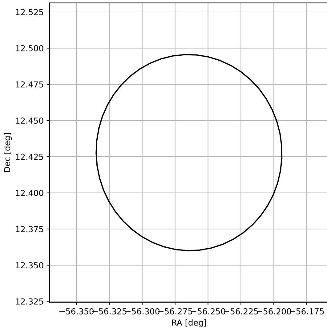
4FGL J2014.9+1225
