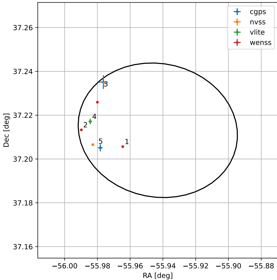
4FGL J2016.2+3712
