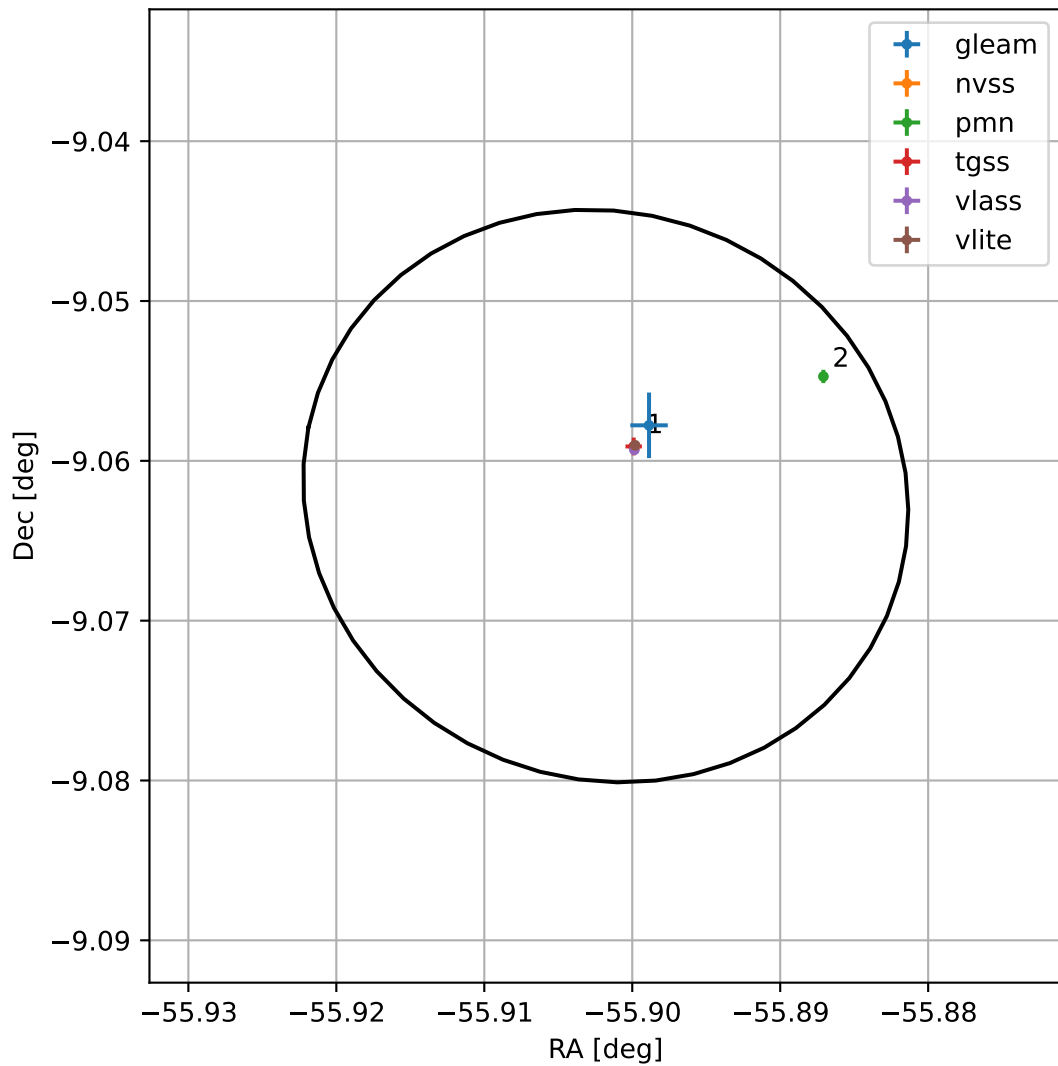
4FGL J2016.3-0903
