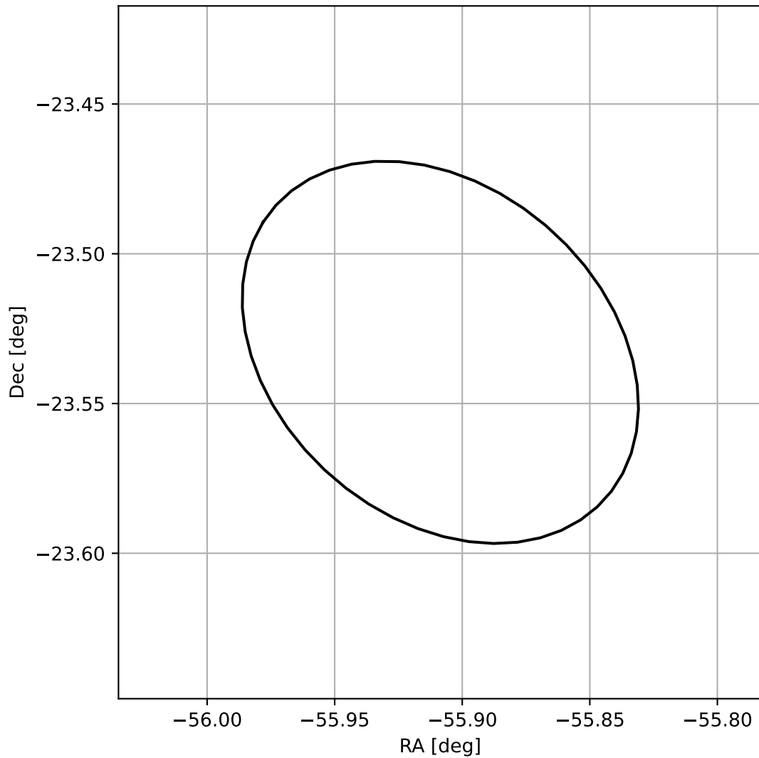
4FGL J2016.3-2331
