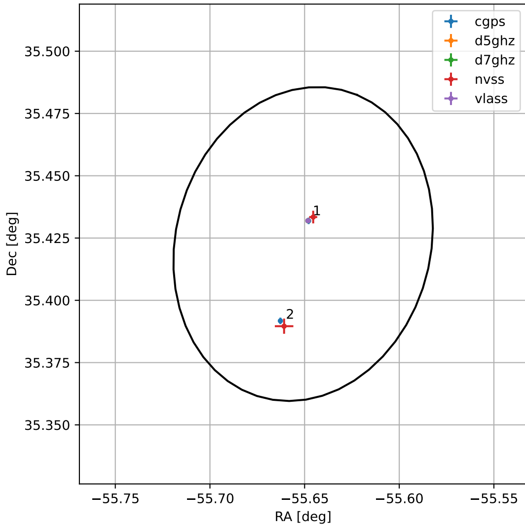
4FGL J2017.3+3525
