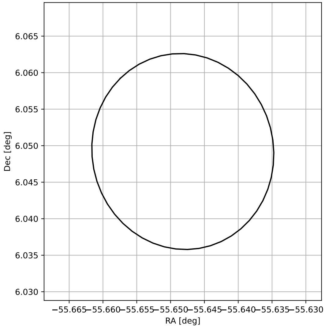
4FGL J2017.4+0602
