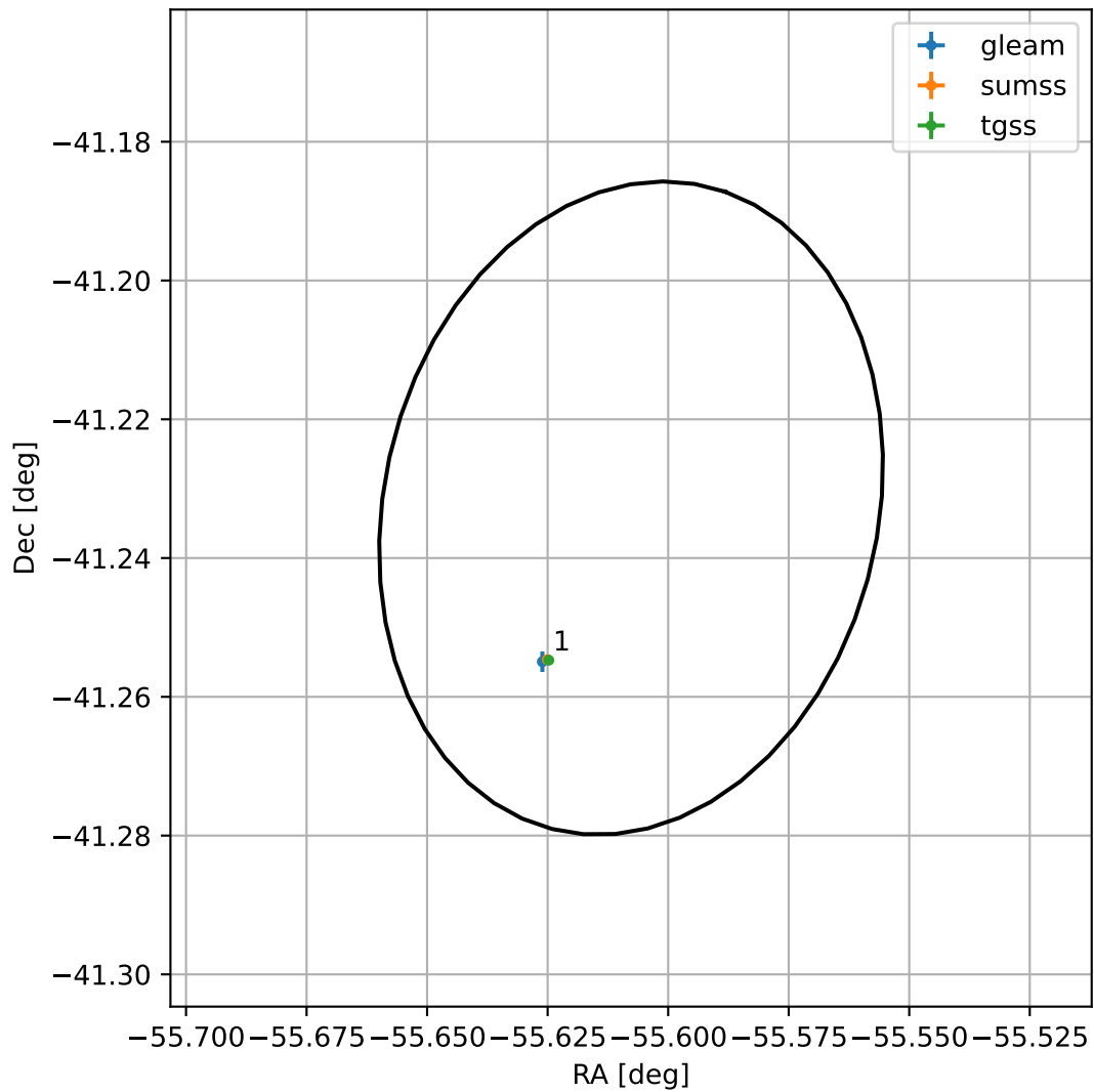
4FGL J2017.5-4113
