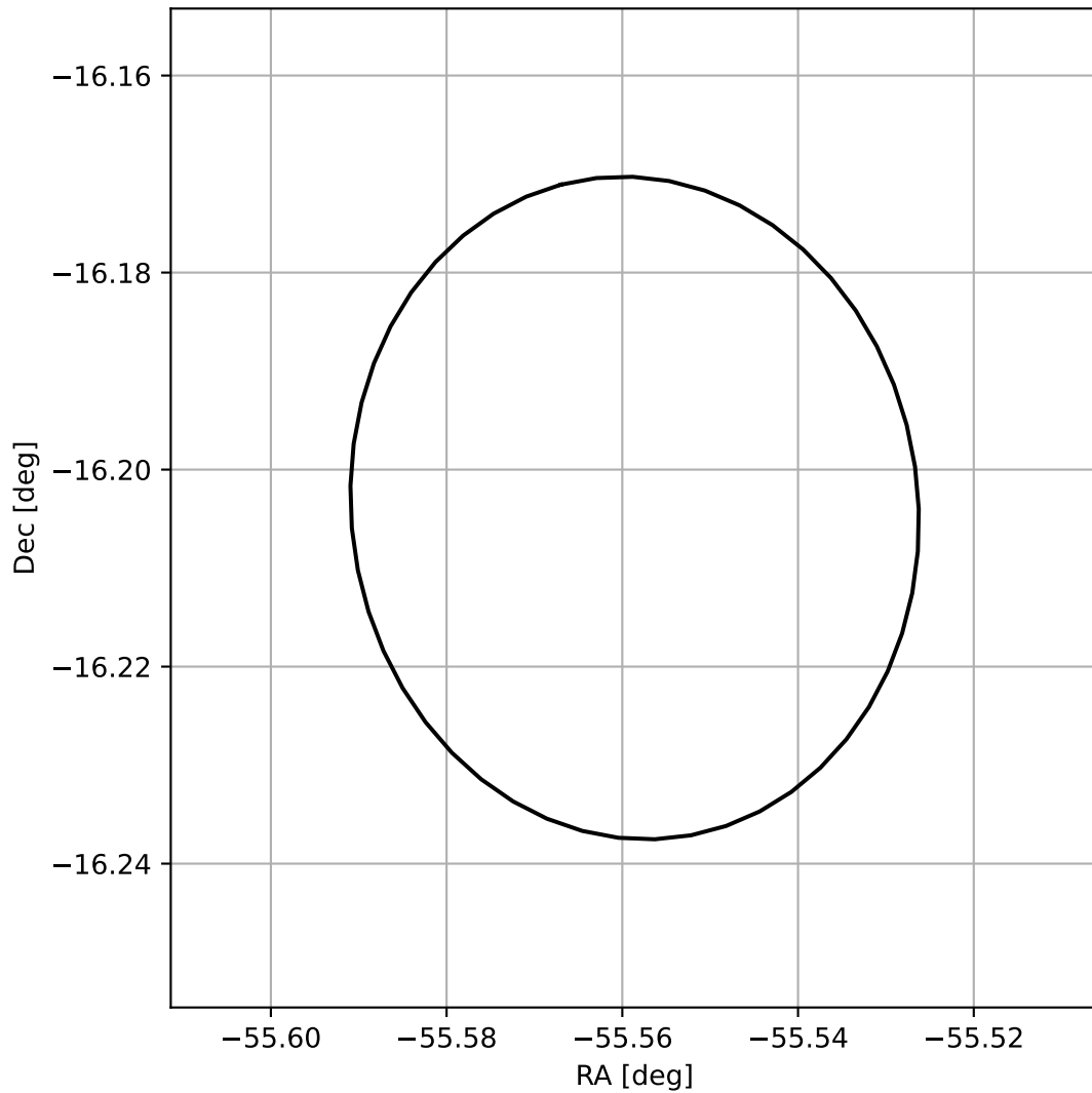
4FGL J2017.7-1612
