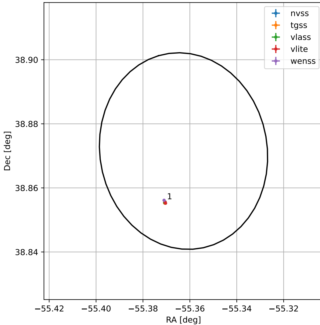
4FGL J2018.5+3852
