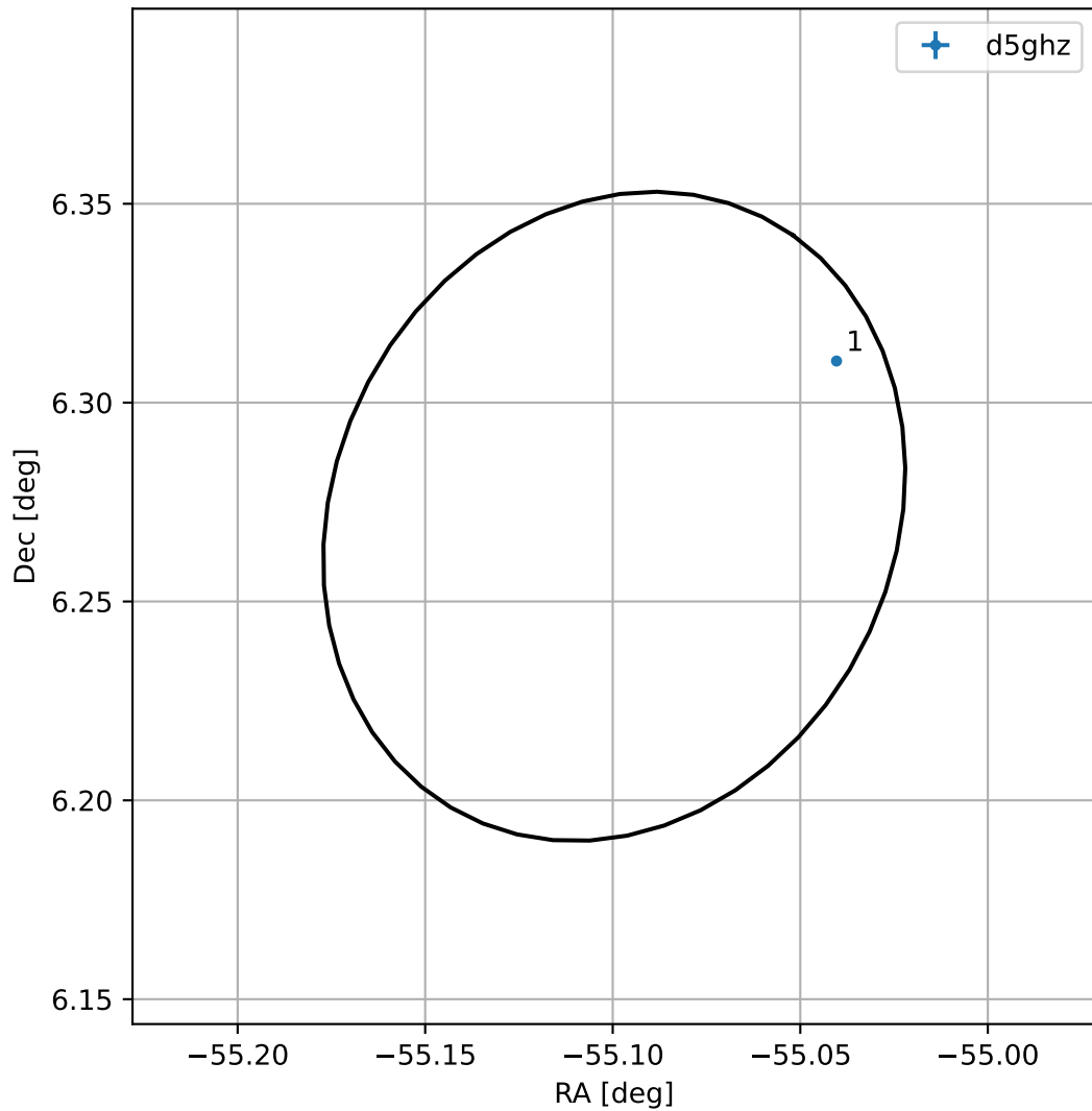
4FGL J2019.6+0616
