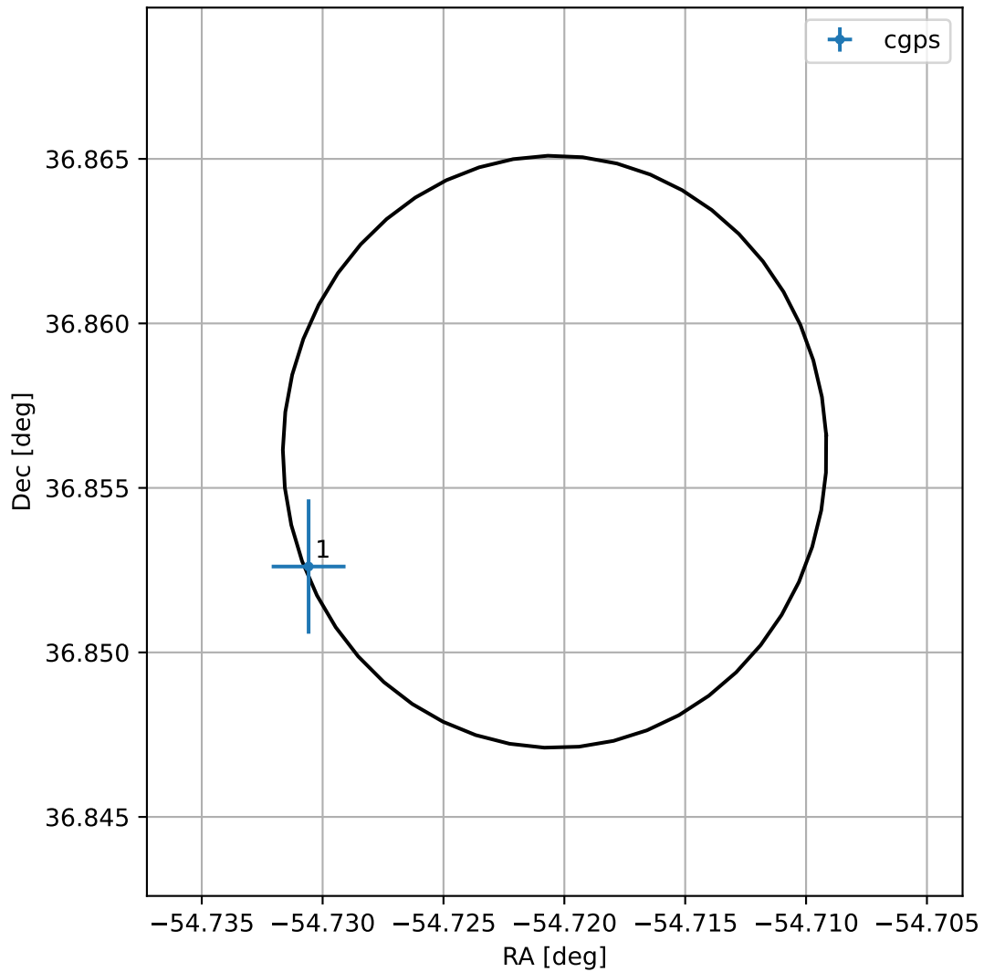
4FGL J2021.1+3651
