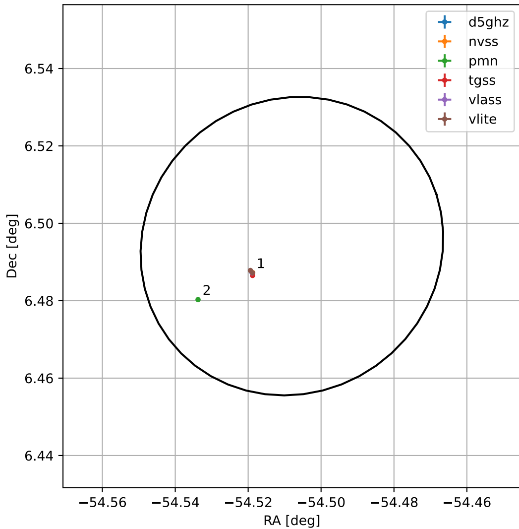
4FGL J2021.9+0629
