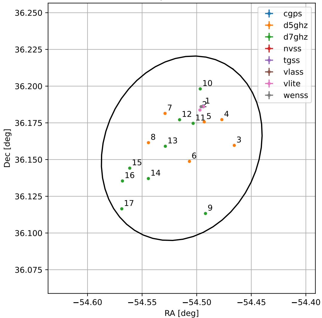
4FGL J2021.9+3609
