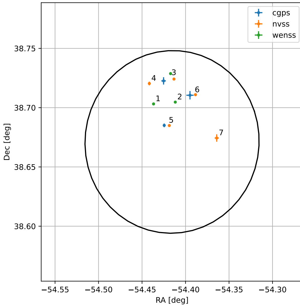
4FGL J2022.3+3840
